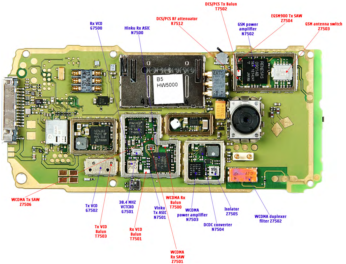
Figure 1 RF key component placement
