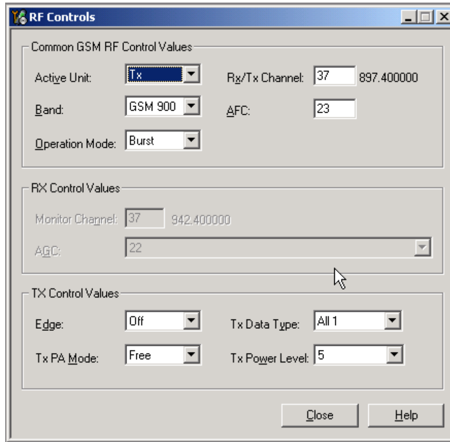
Figure 8 RF Controls window
