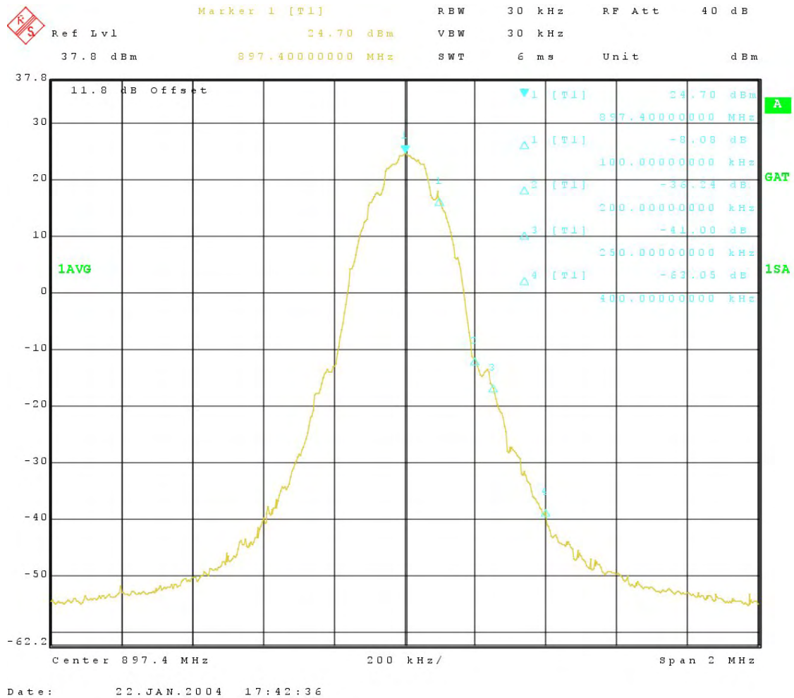
Example of the TX modulation spectrum (GMSK) in EGSM900 band.
