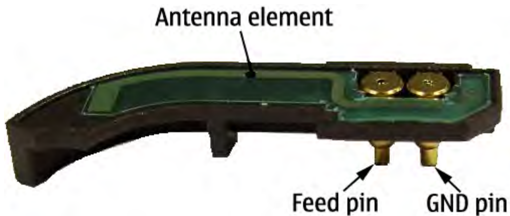
Figure 11 BT antenna
