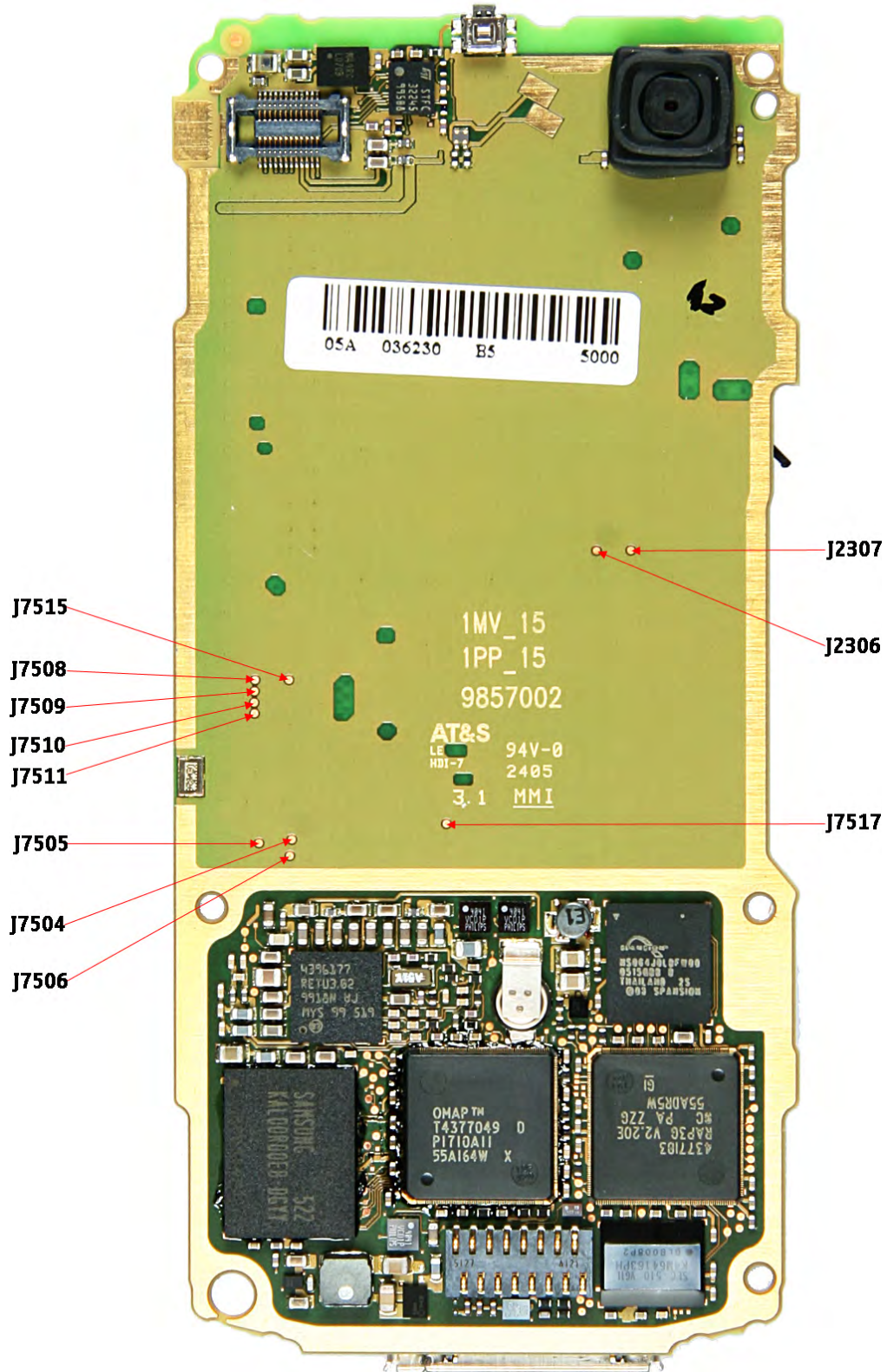
Figure 4 Test points for oscilloscope - top
